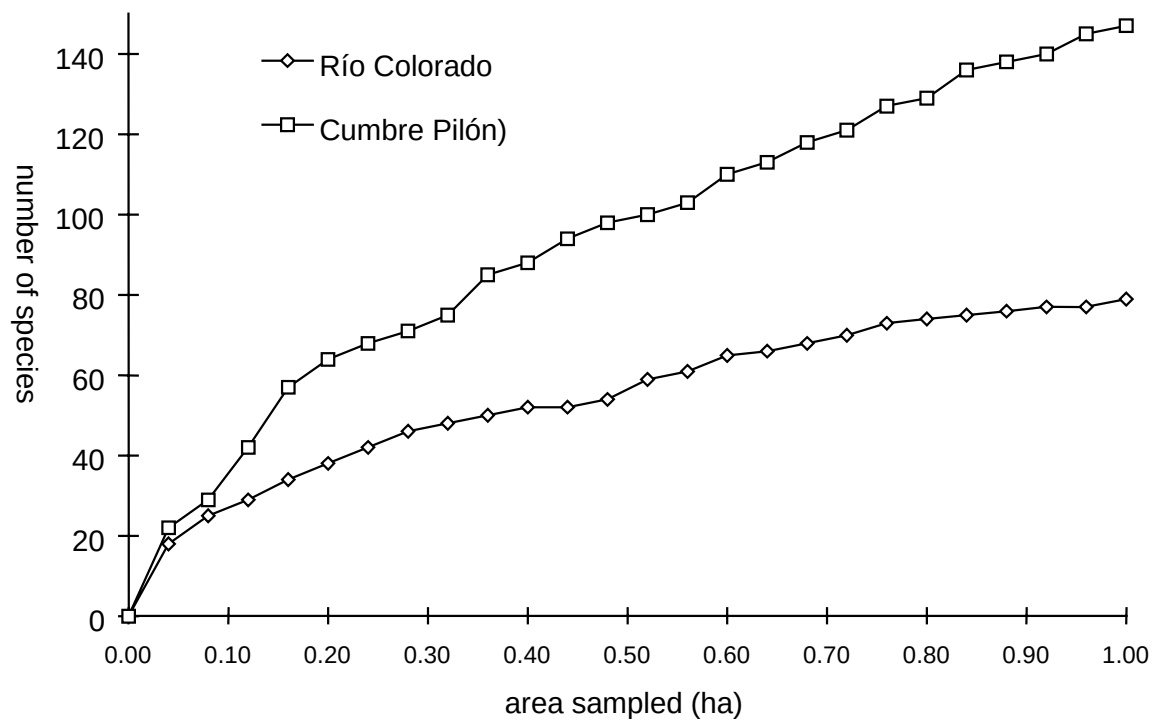
Figure 3. The relationship between tree diversity and sample area for trees with dbh \geq 10 cm dbh for two one hectare plots on the Serranía Pilón Lajas.
