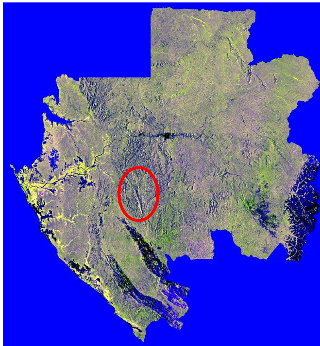
The rift valley visible from a high altitude (map from www-radar.jpl.nasa.gov/africamap/gabon.htm )
